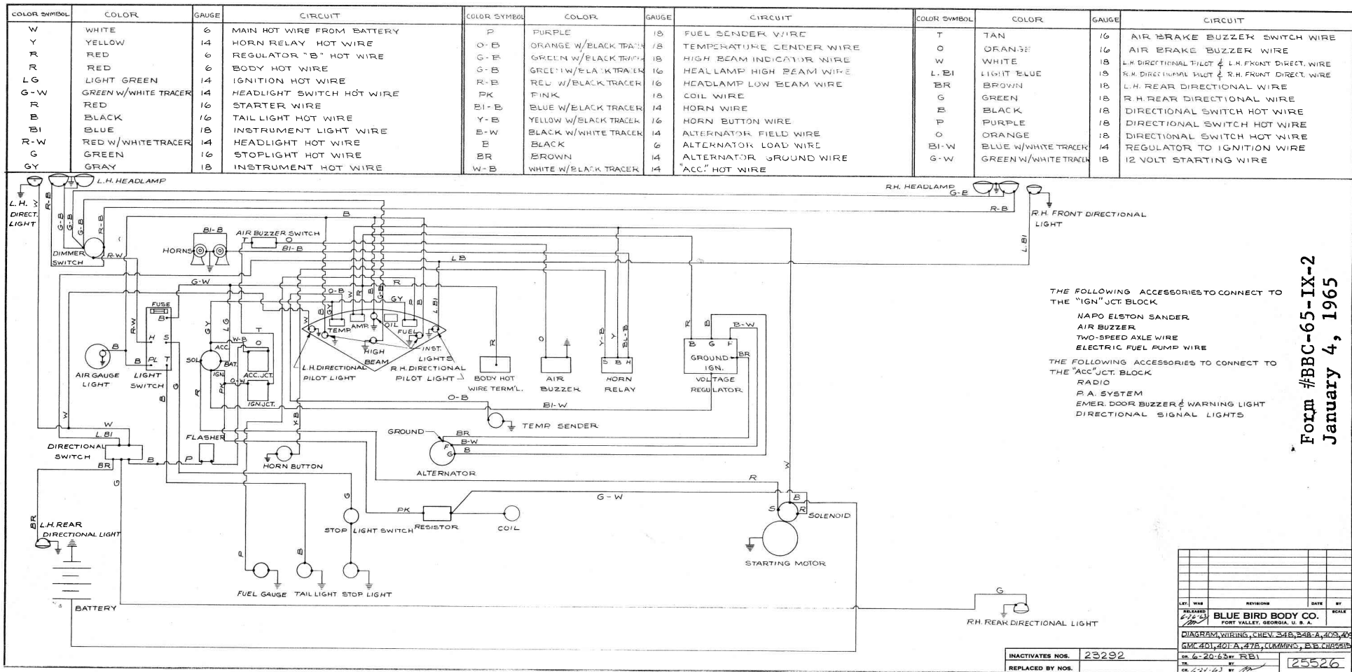
Diagram, Wiring, Chev. 348, 348A, 409, 409A GMC 401, 401A, 478, Cummins
