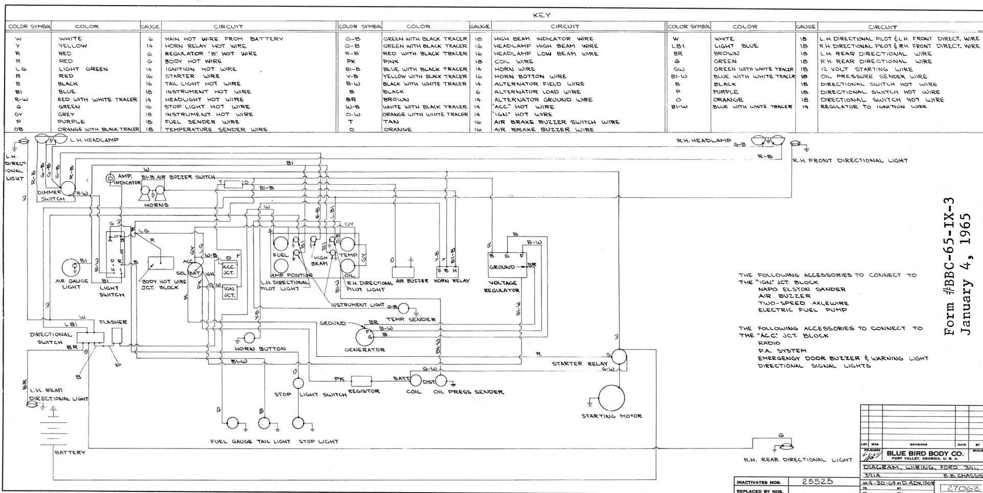
Diagram, Wiring, Ford 391, 391A
