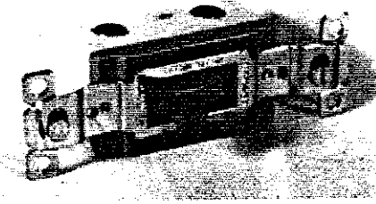
2224434 Switch, Engine Block - 3 Terminals (15A, 120/277 VAC)
