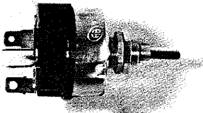
0849414 Switch, Electric Wiper (2 Speed) 0982819 Knob, Wiper Switch
